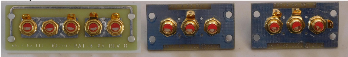
Figure 3-Jack installation, (right channel, red insulator jacks shown)
