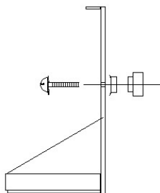
Figure 7-Good Ground Installation
