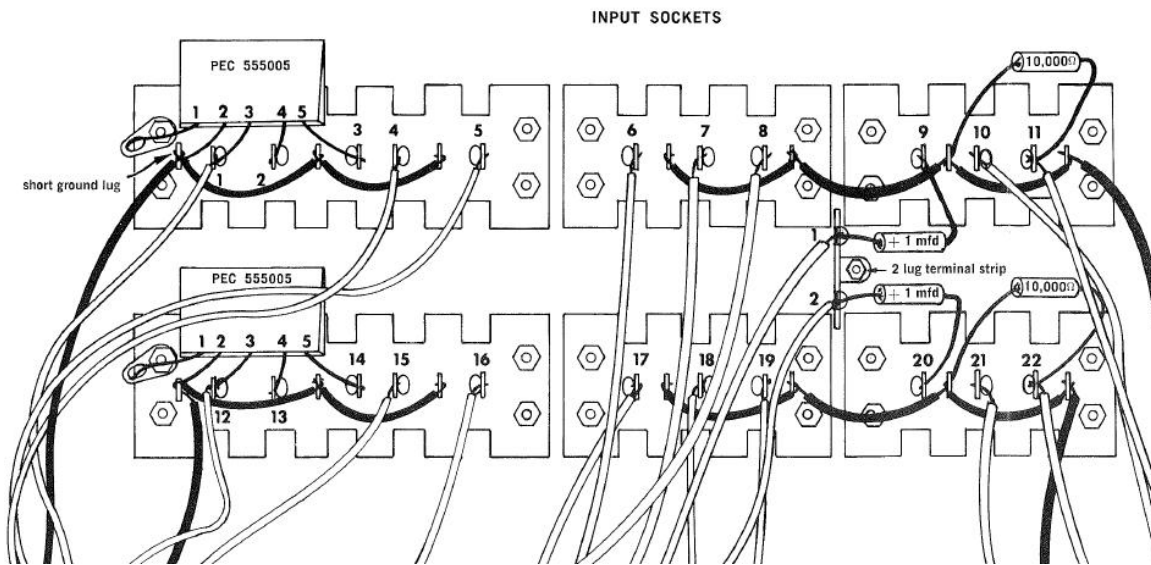
Figure 4-Jack Installation, Rear View (stock arrangement)
