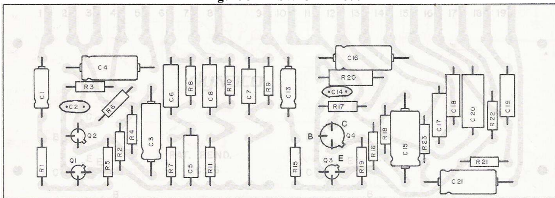
Figure 4-circuit board as seen from solder side. The modification replaces Q4
