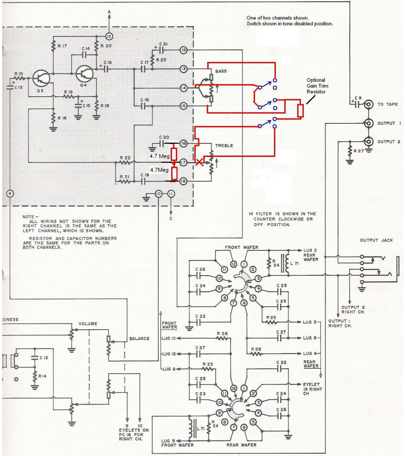
Figure 8-Schematic of the preamp high level stage showing the addition of the tone control switch
