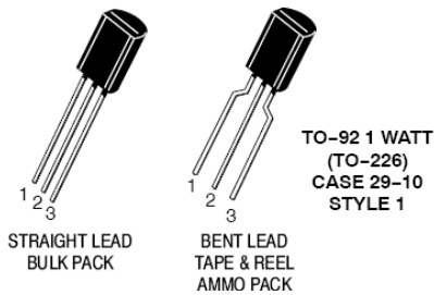
Figure 3-MPSW45A Pinout
