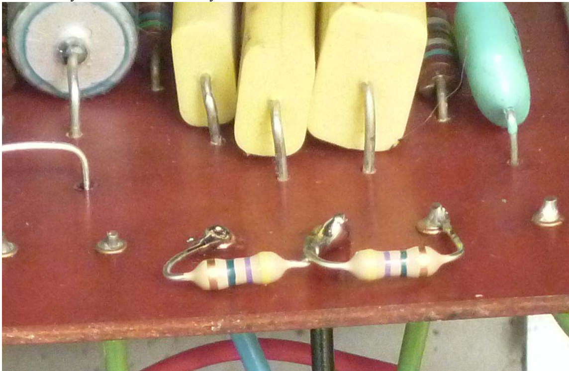
Figure 6-Installing the treble no-click resistors on eyelets 16, 17, and 18
