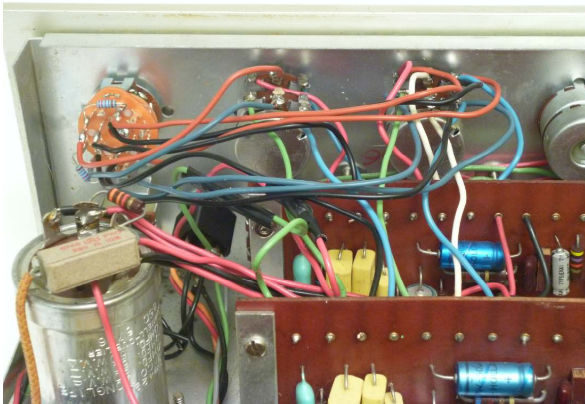
Figure 7-Tone control switch installed and wired to bass control, treble control and PCB's (green wires called out in the assembly directions are blue in the pictures above).
