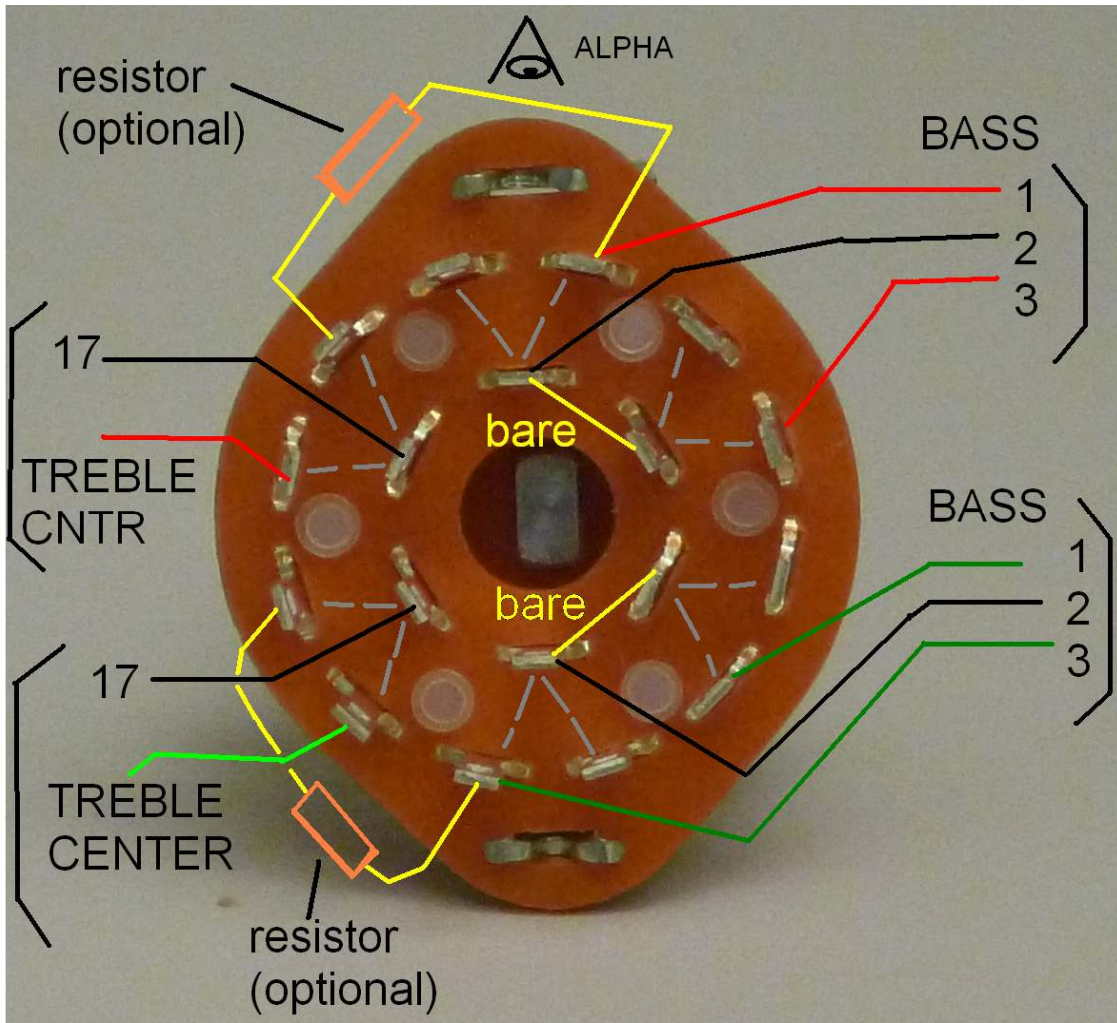
Figure 5-Switch Wiring Diagram. The gray dashed lines indicated relations between poles (center terminals) and throws (outer terminals). These gray lines are not on the actual switch. The gain resistors are optional, and not included with the kit
