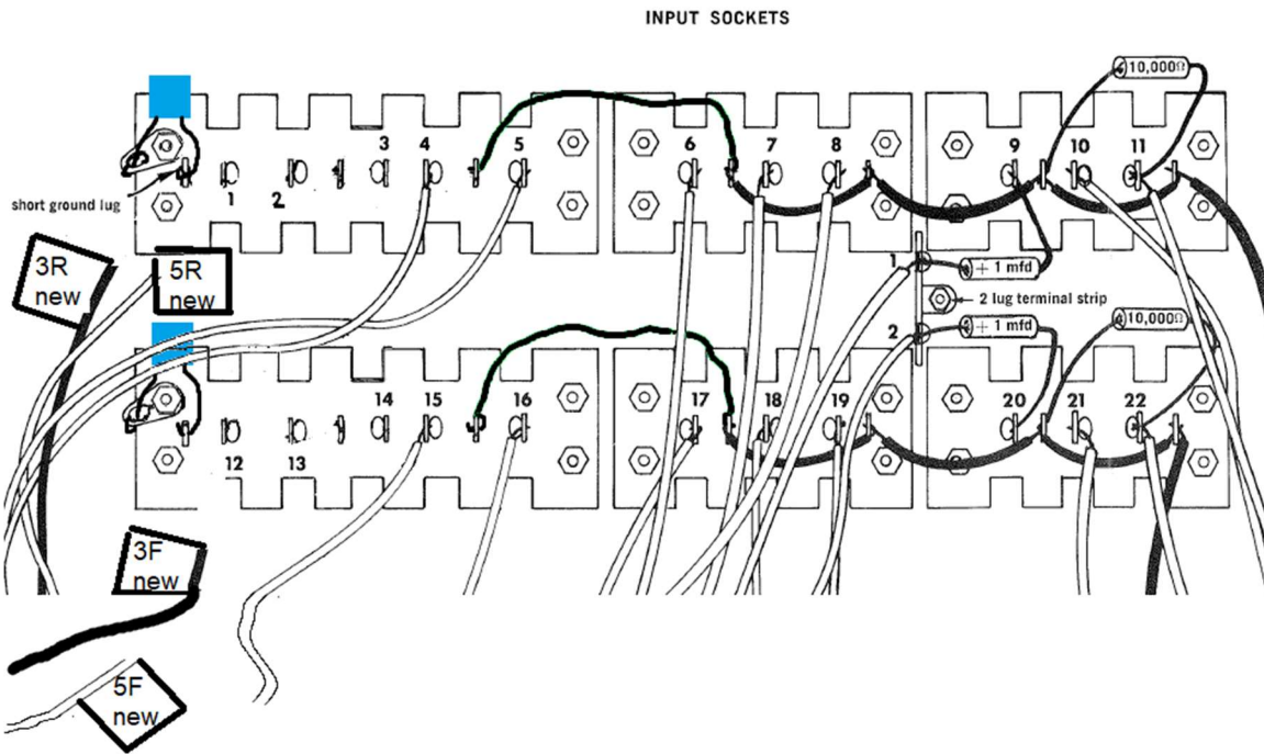
Figure 11-back panel after previous set of tasks and addition of 0.01 uF caps
