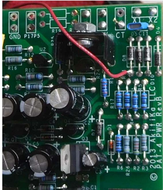
Figure 9-Adding the power good wire to D8's cathode
