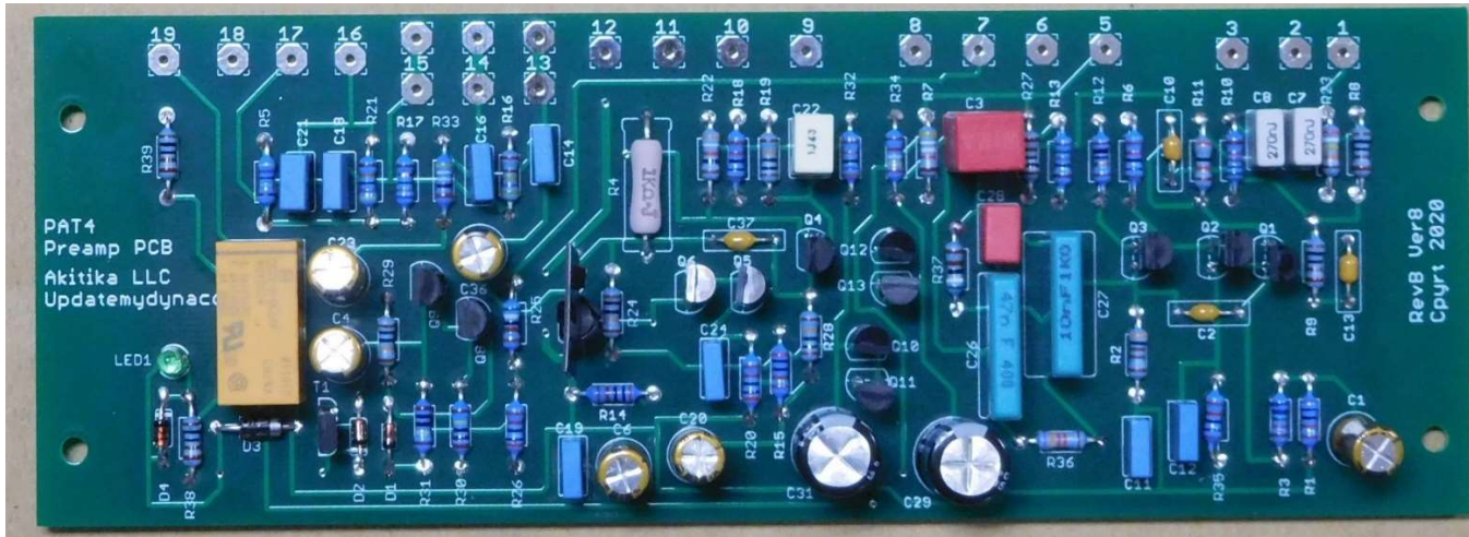
Figure 3-Assembled Single Channel (Rev B Ver8)
