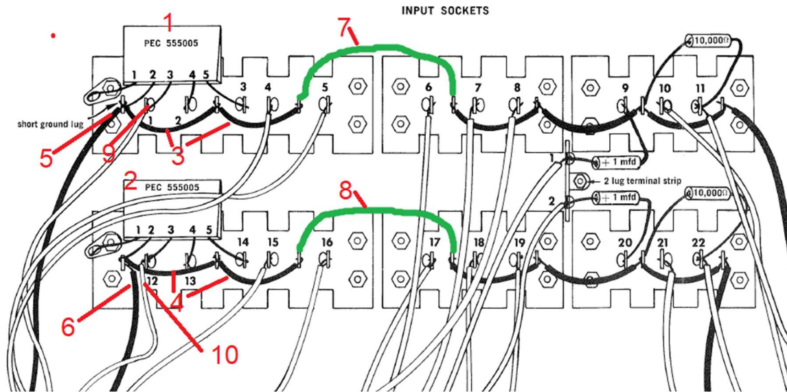
Figure 10-Back Panel wire cuts and ground additions
