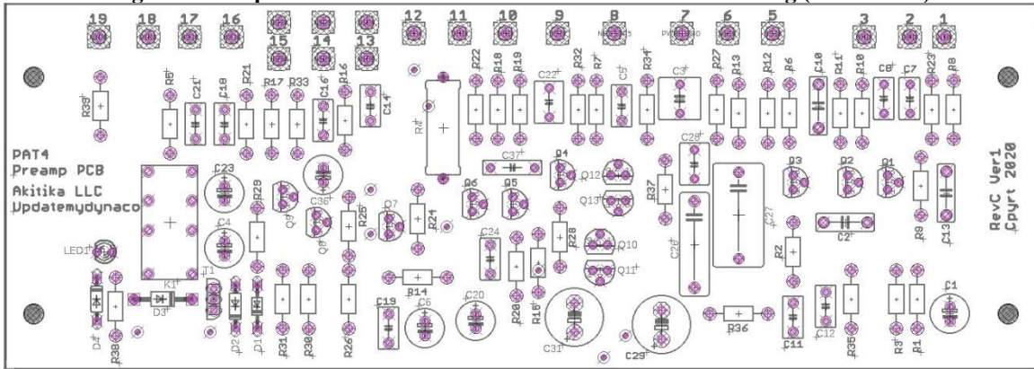
Figure 2-Component side of the PAT4RENEW PCB before loading (RevC Ver1)
