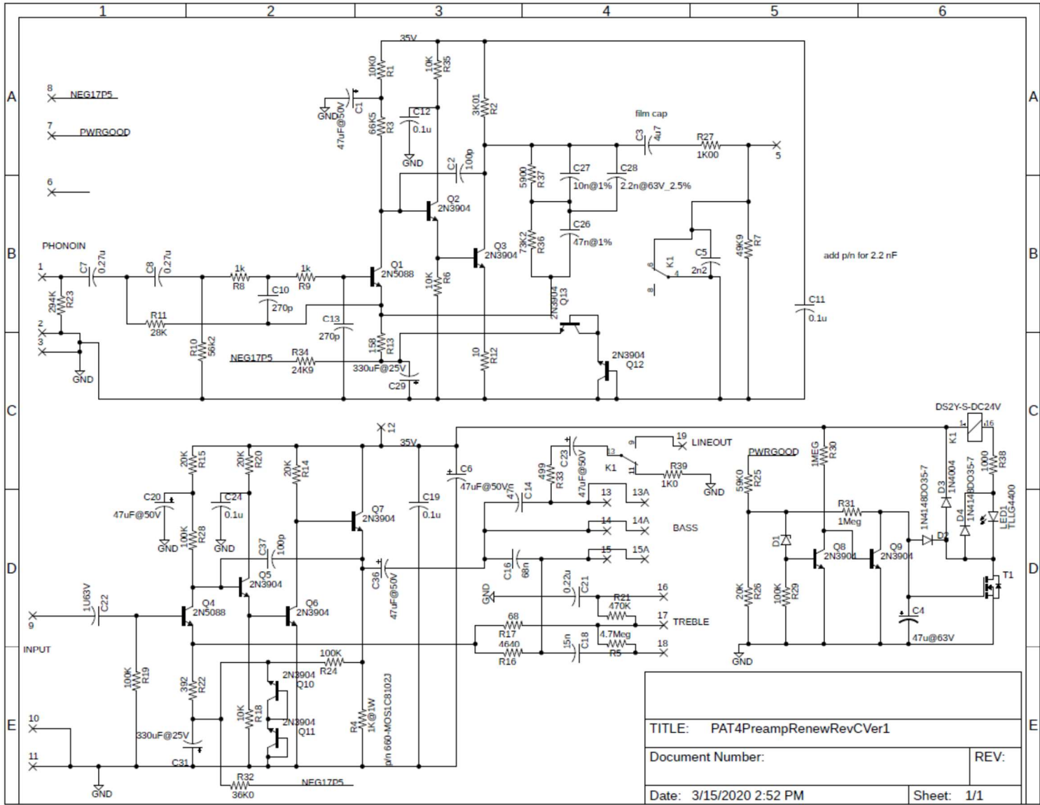
Figure 14-Schematic of the PAT4Renewal Board Note that RevCVer1 PCBs add a place for C5, not populated, in parallel with R7
