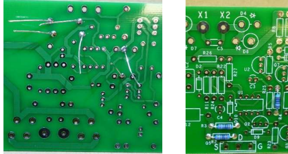
Figure 5-Installing resistors
