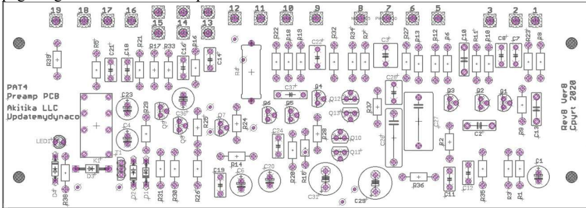
Figure 1-Component side of the PAT4RENEW PCB before loading (RevB Ver8)
