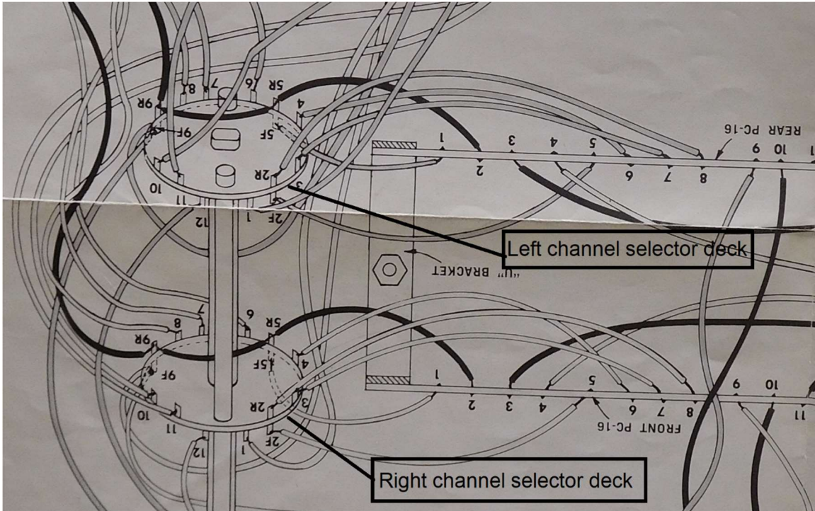
Figure 12-Original switch wiring
