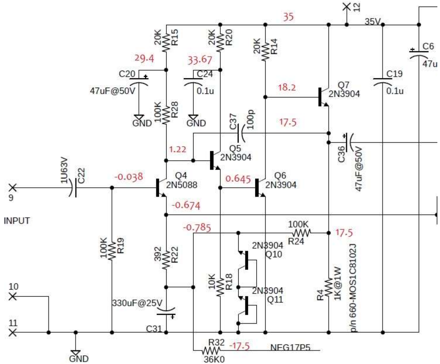
Figure 15-DC voltages on the line stage
