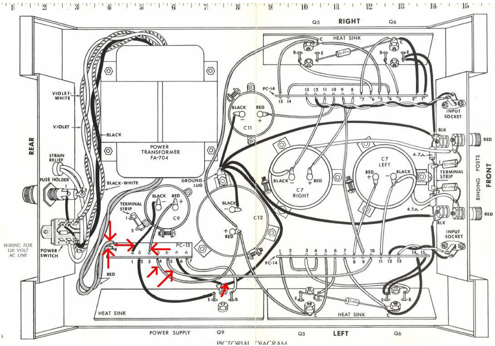
Figure 5-Location diagram for cutting wires
