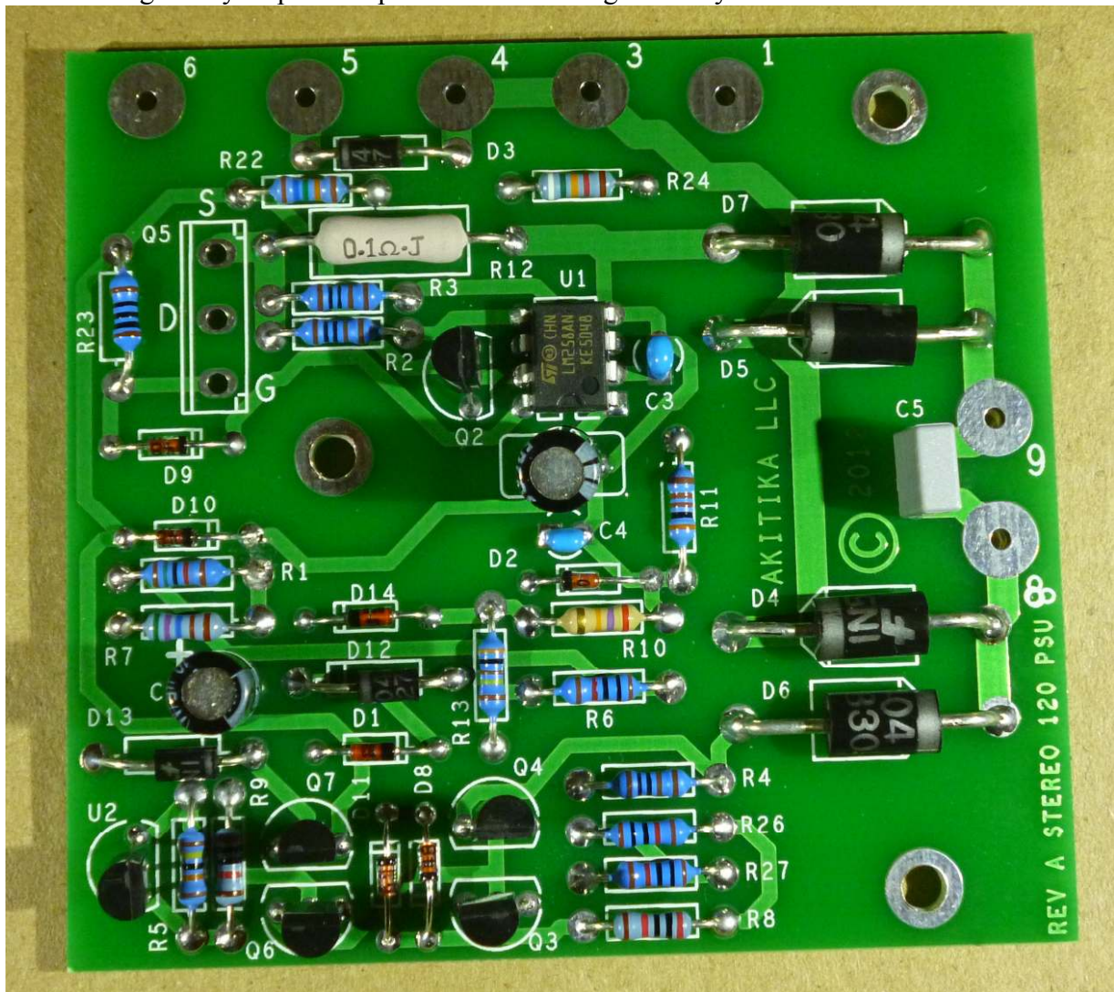
Figure 3-Completed Circuit Board (to this point). Your R10 will look different.
