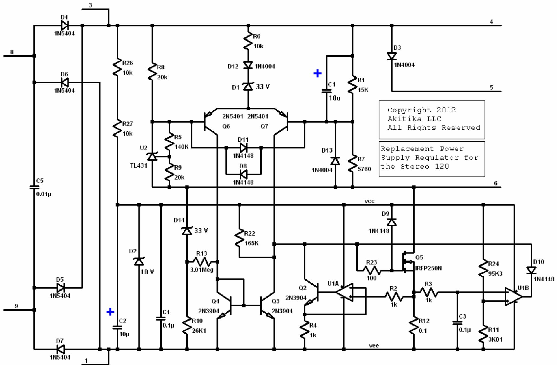
Figure 15-Schematic of amplifier module
