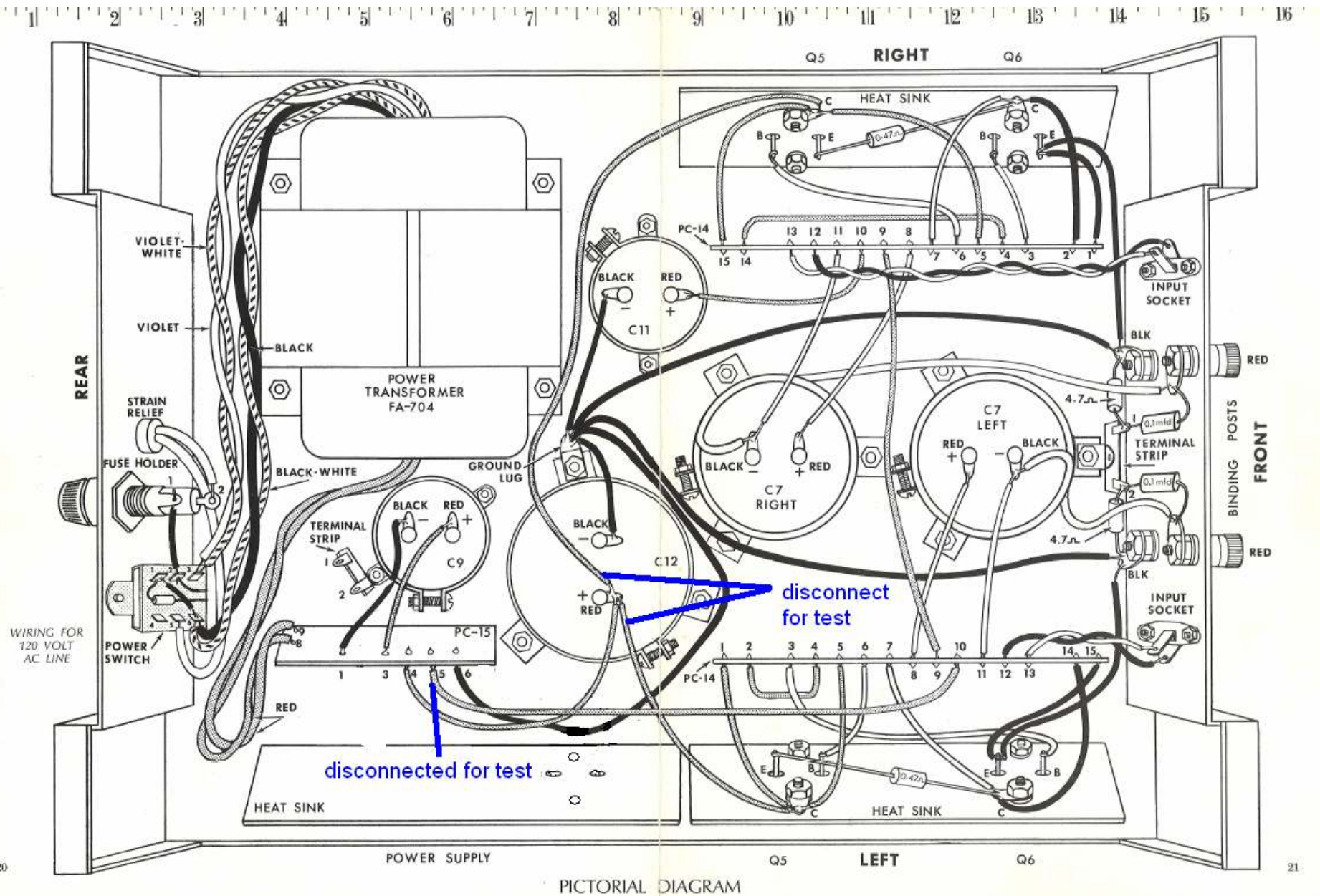
Figure 12-Original Amplifier Modules: Final wiring, showing which wires are disconnected for power supply test
