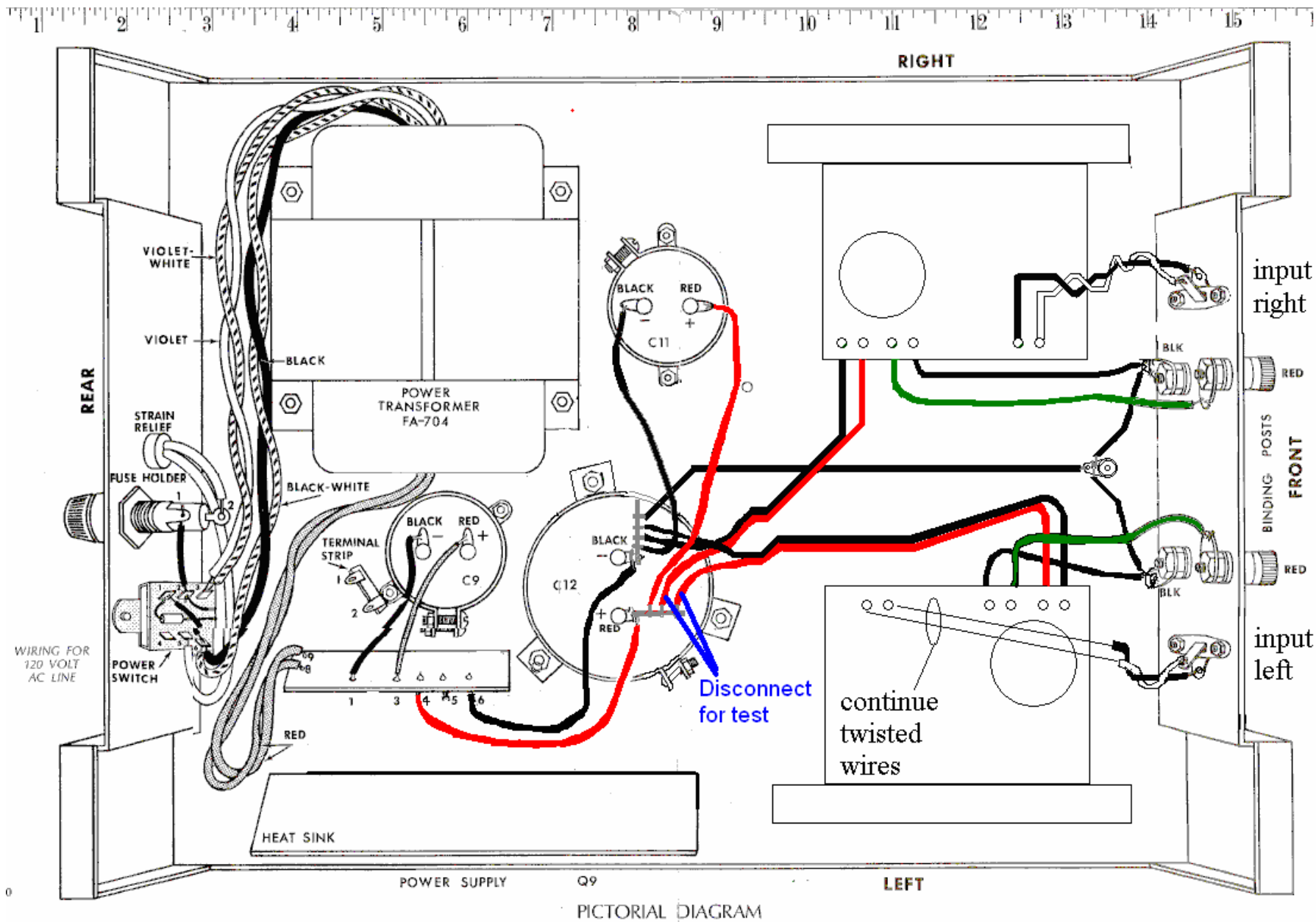
Figure 13- Upgraded Amplifier Modules: Final wiring, showing which wires are disconnected for power supply test
