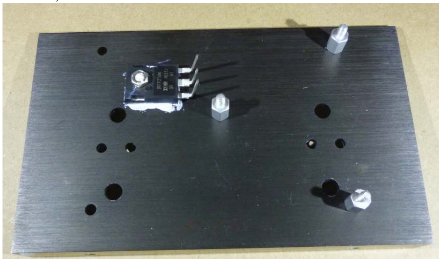
Figure 9-fasten Q5 to the heat sink as shown
