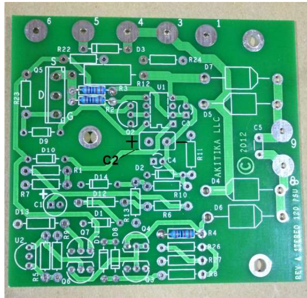
Figure 2-Black text shows proper C2 location and polarity
