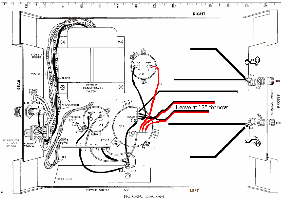
Figure 20-Rewiring the Power and Half the Grounds
