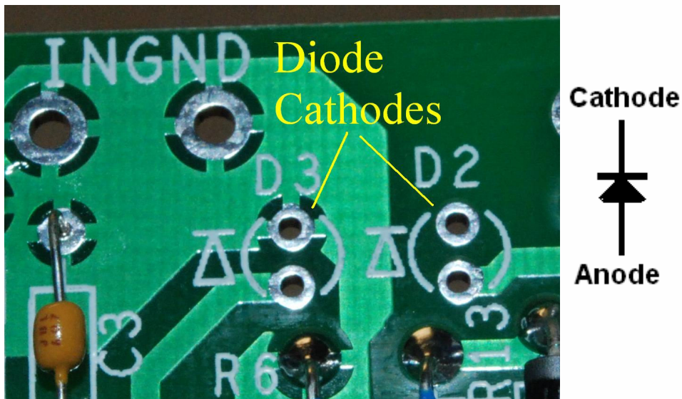
Figure 11-showing LED cathode orientation
