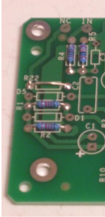
Figure 10-Zero Ohm R22 installation detail
