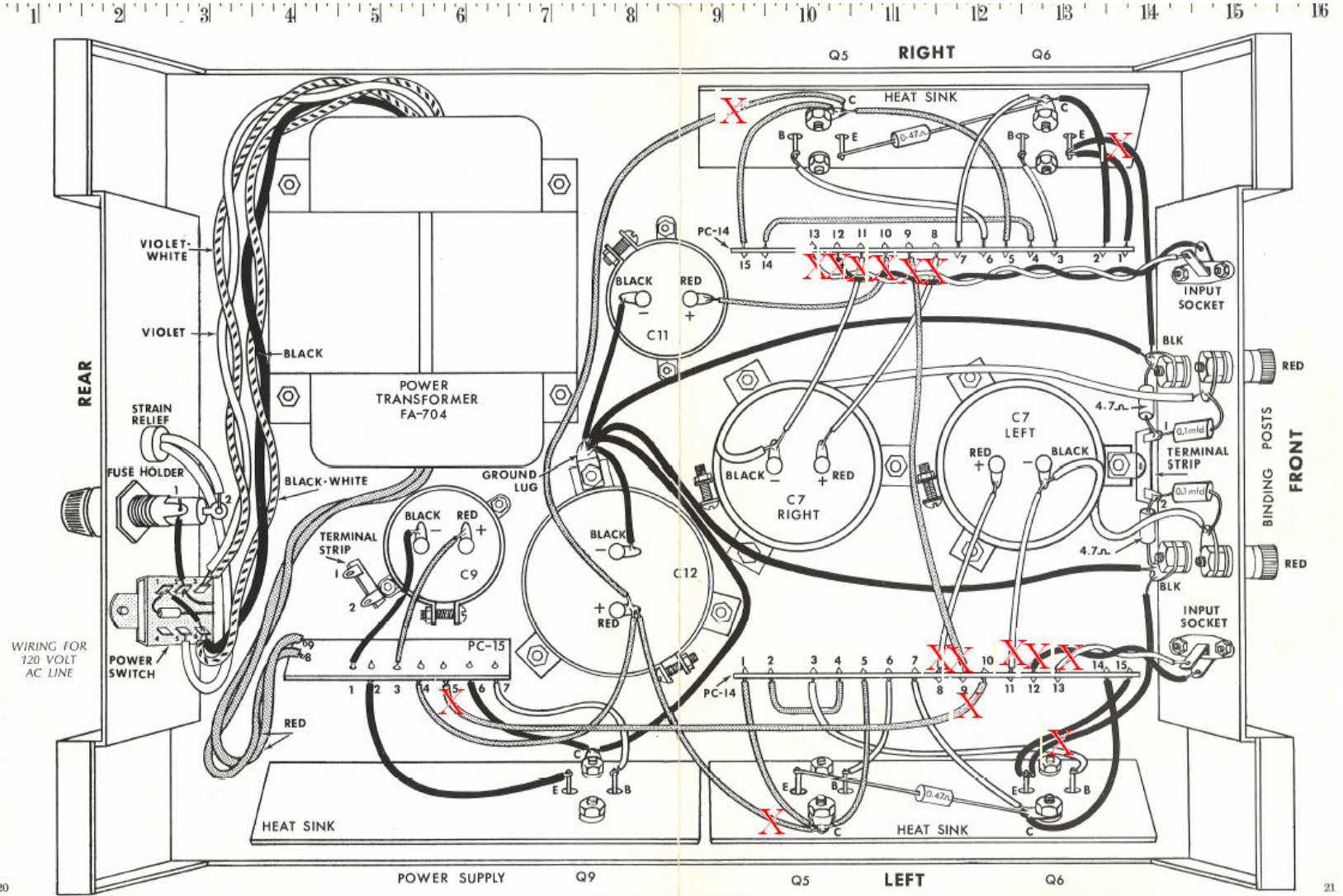
PICTORIAL DIAGRAM
