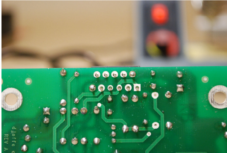
Figure 16-LM3886 installation step three, just the corner pins are soldered
