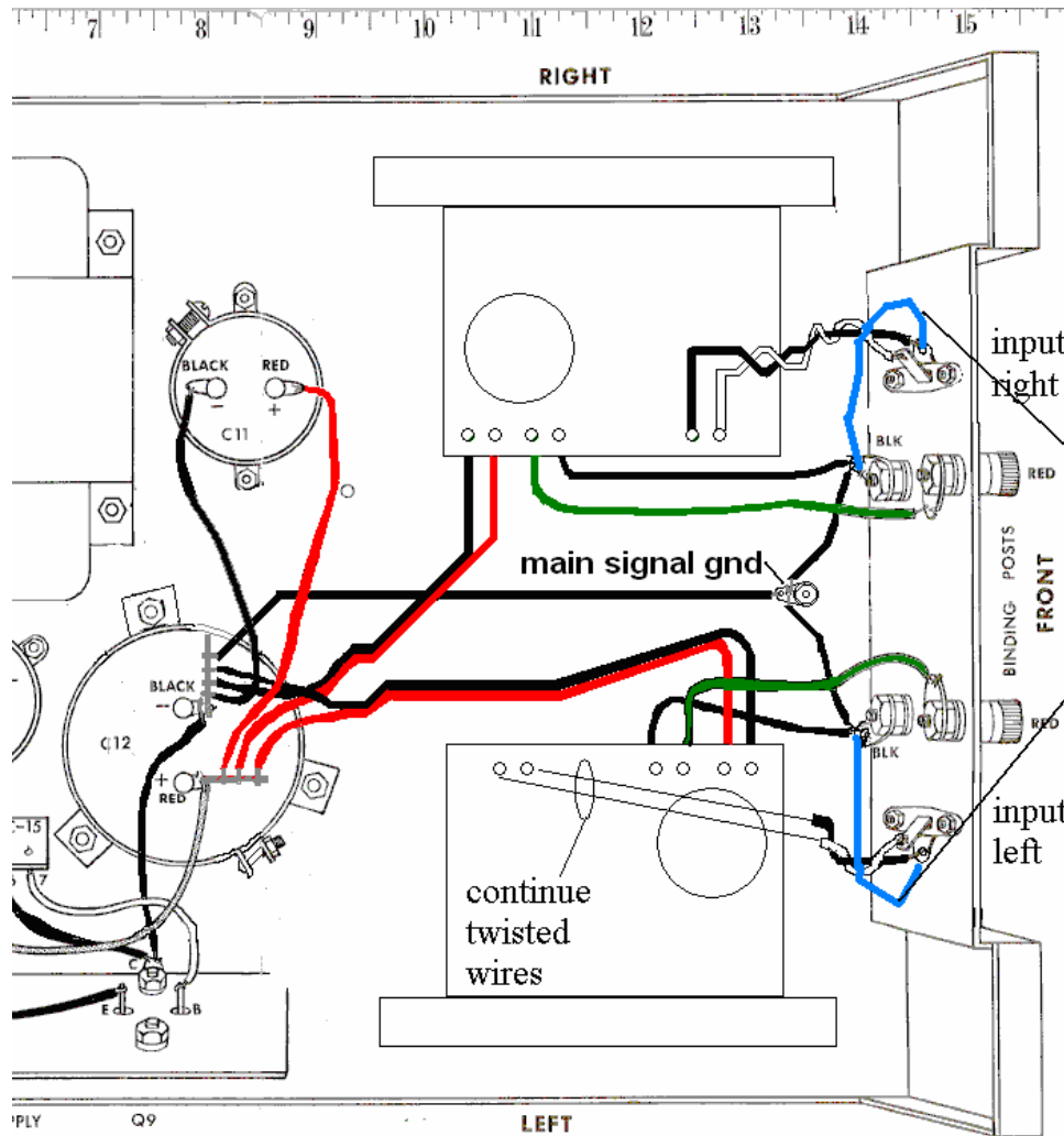
PICTORIAL DIAGRAM
