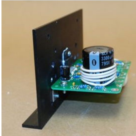
Figure 19-a completed amplifier module
