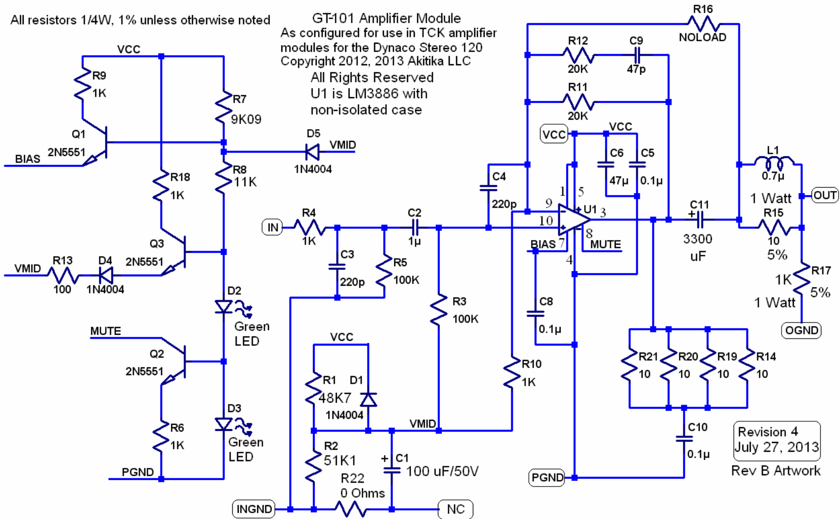
Figure 22-Schematic of amplifier module
