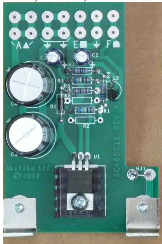
Figure 9-Close up of Assembled Circuit Board
