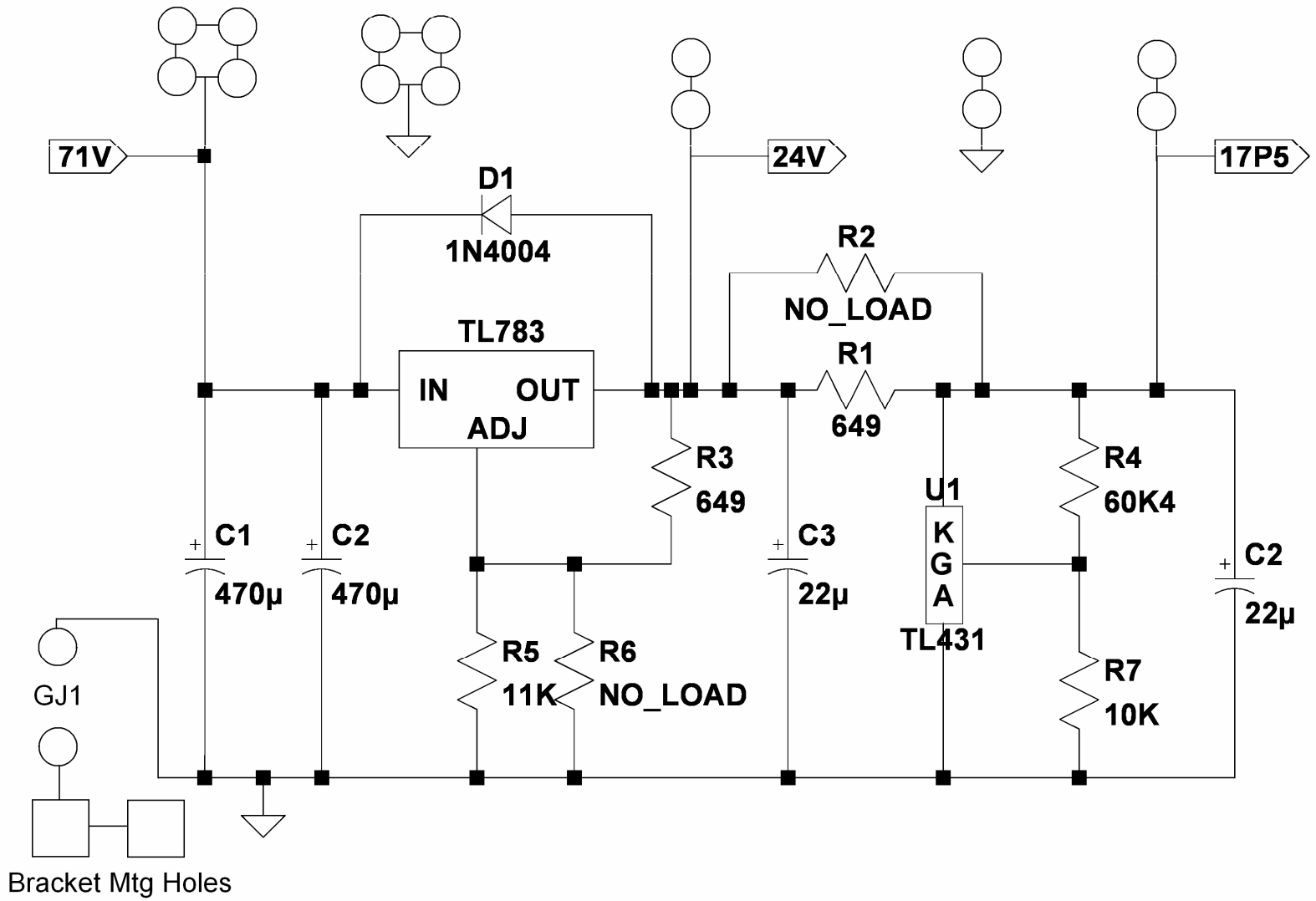
Figure 10-Schematic of C11 Replacement Electronically Regulated Power Supply for SCA-80
